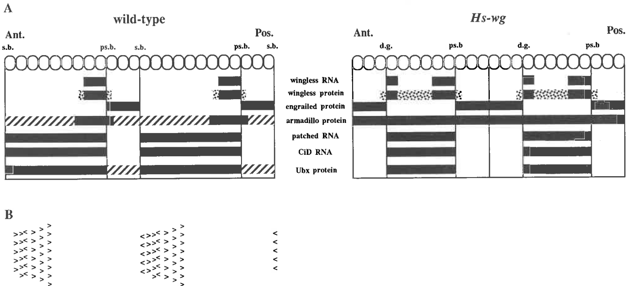
Fig. 7. Schematic representation of the expression pattern of several segmentation genes and cuticle phenotype in wild type and HS- wg . (A) Expression of segmentation and selector genes in a stage 10/11 wild-type and HS- wg embryo, 3 hours after heatshock (Materials and methods). A schematic drawing of two adjacent segments is shown. At this stage of embryogenesis, each segment is about 12 cells in width. The domain of expression of each gene is depicted by the black boxes. Directly after heatshock in HS- wg embryos wingless is expressed uniformly throughout the segment. Here, wingless expression is shown 3 hours after heatshock; the HS- wg RNA has disappeared and an ectopic domain of endogenous wingless RNA is observed just posterior to a deep groove. This deep groove is formed in HS- wg embryos posterior to the new engrailed domain (Fig. 4E). The wingless protein is detected at a low level between the ectopic wingless domain and the normal wingless stripe (Fig. 4B), most likely due to spreading of the protein (spread protein is indicated as dots). In wild-type embryos, the protein can also be detected outside the cells where it is made (shown by the dots; Van den Heuvel et al., 1989). engrailed in HS- wg embryos has broadened in the posterior direction, spanning half a segmental unit (Fig. 4E), while the high level of armadillo protein, normally only found in the wingless domain (Fig. 6A), has extended to the whole segment (Fig. 6B). The low basal level of armadillo protein in wild-type embryos is shown by stripes. In HS- wg embryos patched RNA, cubitus interruptus Dominant RNA and Ubx protein expression seem to correlate with and perhaps follow the altered distribution of engrailed . In the wild type, engrailed represses patched (Hidalgo and Ingham, 1990), cubitus interruptus Dominant (Eaton and Kornberg, 1990) and Ubx (Martinez-Arias and White, 1988) in a temporally and spatially distinct pattern. In HS- wg , where we observe an expansion of engrailed , we see a retraction of patched (Fig. 6F) and cubitus interruptus Dominant (Fig. 6I). Ubx is down-regulated in the anterior half of parasegments 7-12, where engrailed is expressed at a high level (Fig. 6L). The lower level of Ubx in the posterior compartment of the wild-type segment is indicated by the stripes. (Abbreviations: Ant., anterior; Pos., posterior; s.b., segment border; ps.b., parasegment border; d.g., deep groove.) (B) Location of denticle belts and naked cuticle in wild-type and HS- wg larvae. In wild-type embryos, abdominal segments are characterized by a belt of denticles in the ventral cuticle of which the first row is in the posterior segmental compartment of the preceding segment, while the other approx. six rows are present in the anterior part of the anterior segmental compartment. The position of the larval belts is shown relative to the embryonic gene expression patterns in A. The more posterior part of the anterior segmental compartment of the larval segment is naked, corresponding to the region where wingless is expressed in the embryonic segment. In HS- wg embryos the denticle belts are lost, resulting in a complete naked segment.
